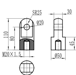
叉销端GA
