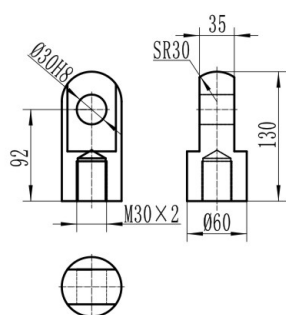
叉销端GA
